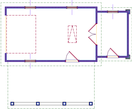
GARAGE PLAN
