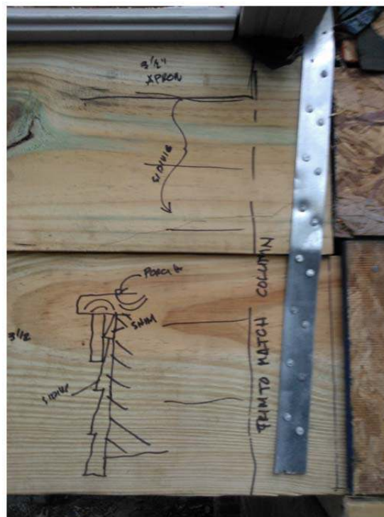
Instructions for trim below Porch Floor & Strapping @ new-existing joint
