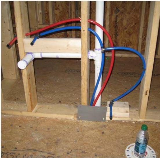
Neat well secured Plumbing Rough-in
